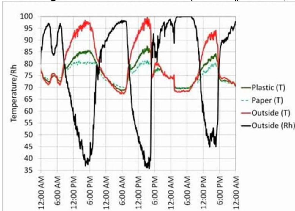
Figure 3. Inside/Outside house temperatures (plastic and paper pads)
