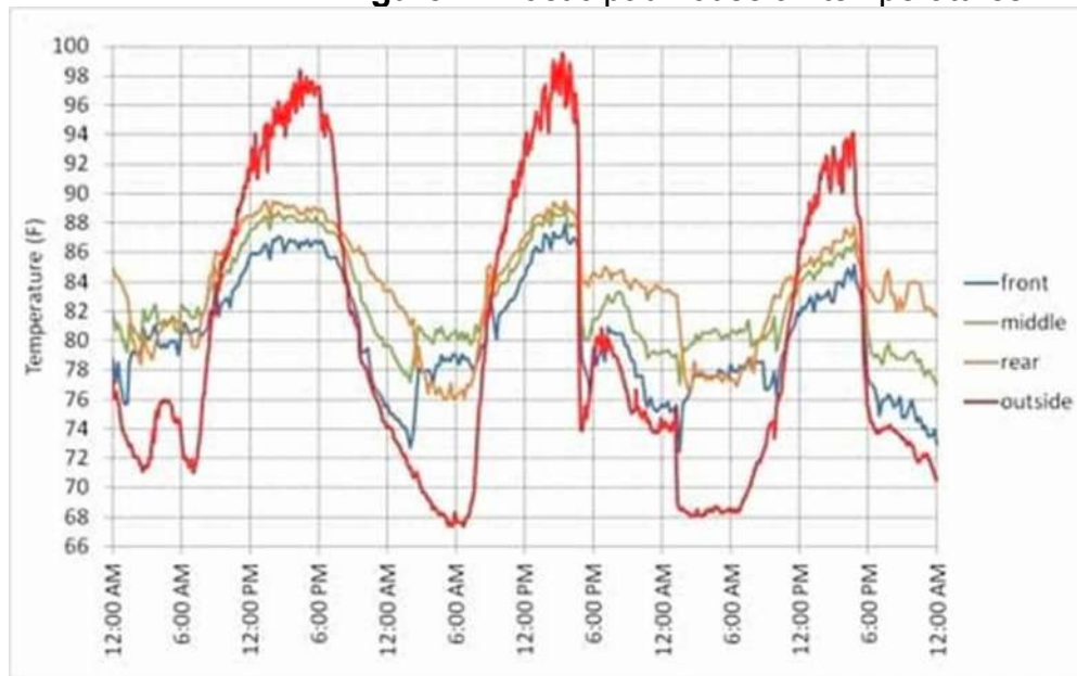
Figure 8. Paper pad house air temperatures
